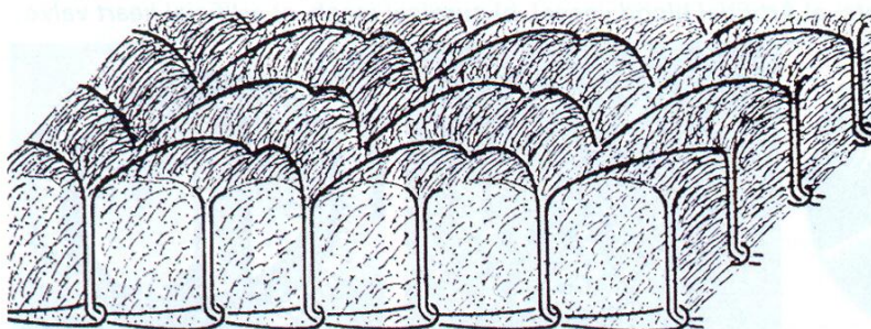
Figure 5: Stitch bonded fabric (Maliwatt)
