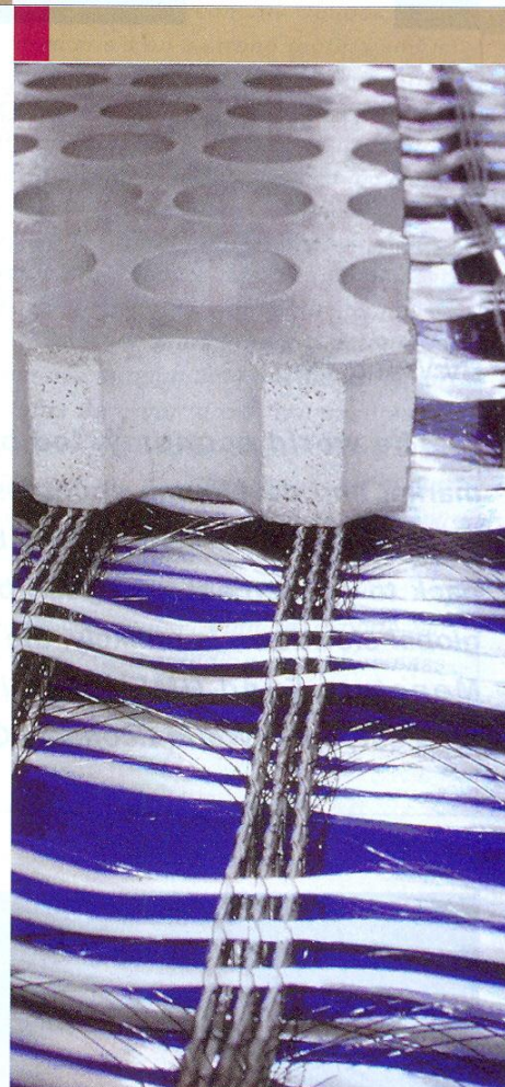
Figure 8: Warp knitted fabric for reinforcement of concrete slab
