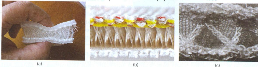
Figure 4: Spacer fabrics. a) Raschel, b) circular knitted, c) V-bed flat knitted
